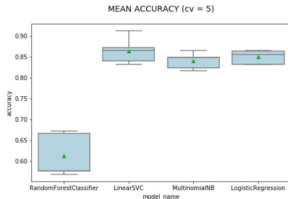
Fig. 2. Accuracy Graph.
