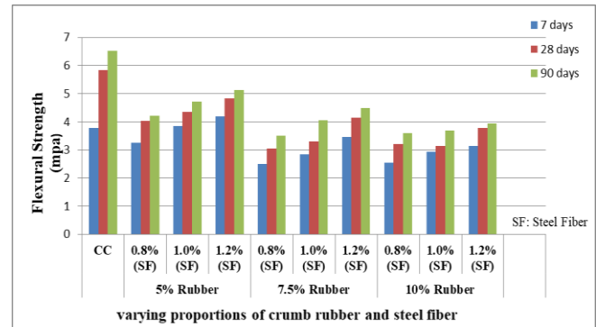
Fig. 10. Flexural strength of RSFC
