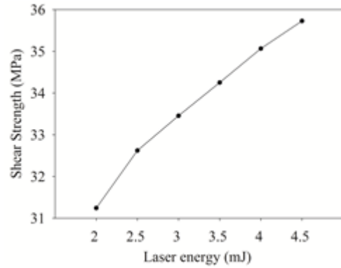
Fig. 10. Shear strength in this research of the effect of laser energy
