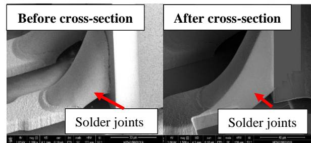
Fig. 7. The cross-sectional view of solder joints in HGA
