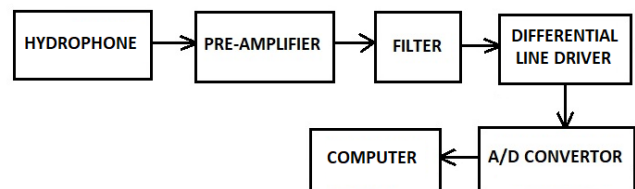
Fig.5. Architectural idea for Autonomous Underwater Vehicle (AUV) Communication System
