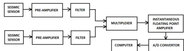
Fig.4. Architectural Block Diagram of Seismograph
