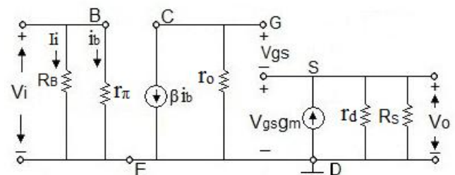
Fig.6. Small Signal AC Equivalent of the Proposed Amplifier (Circuit-2)
