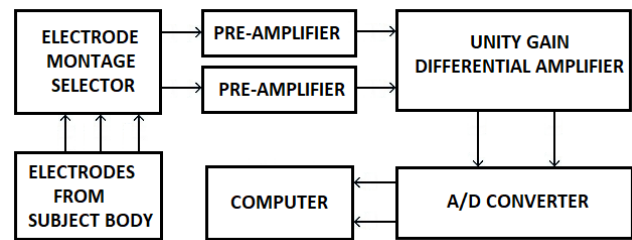
Fig.3. Architectural Block Diagram of Electroencephalogram (EEG)
