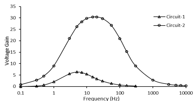
Fig.2. Frequency response of the Circuits under discussion
