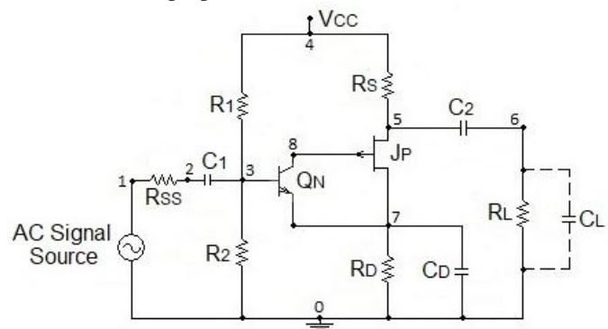
Fig.1. Describing basic circuit structure of the amplifiers under discussion
