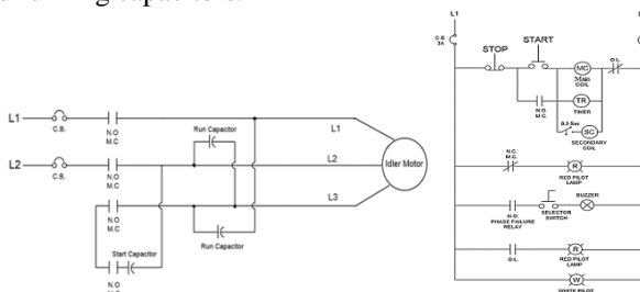
Fig 1. Power and Control Circuit of Idler Motor
