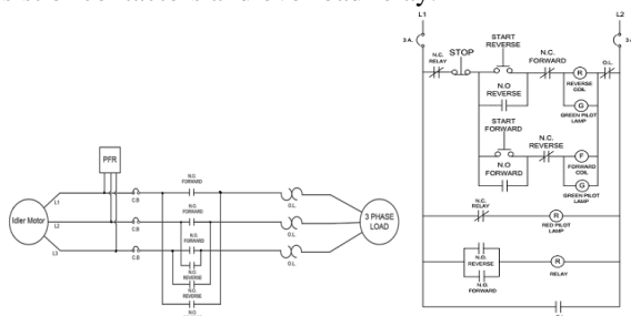
Fig 2. Power and Control Circuit of the Forward-Reverse
