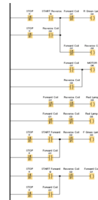
Fig 4. Control Circuit of the Forward- Reverse Simulation
