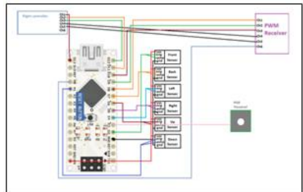
Figure: Collision avoidance system
