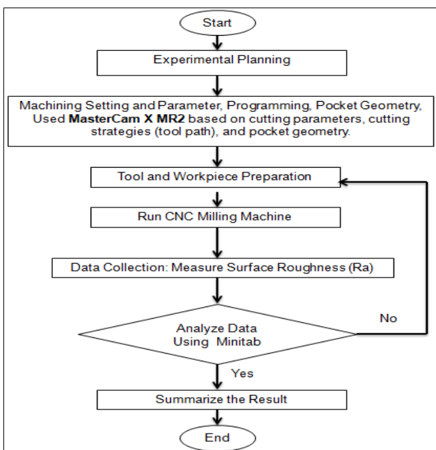
Fig. 1. Experiment Workflow
