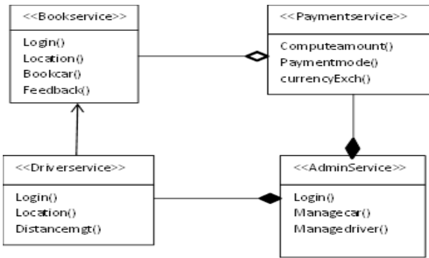
Figure 1: Taxi Service UML interface diagram
