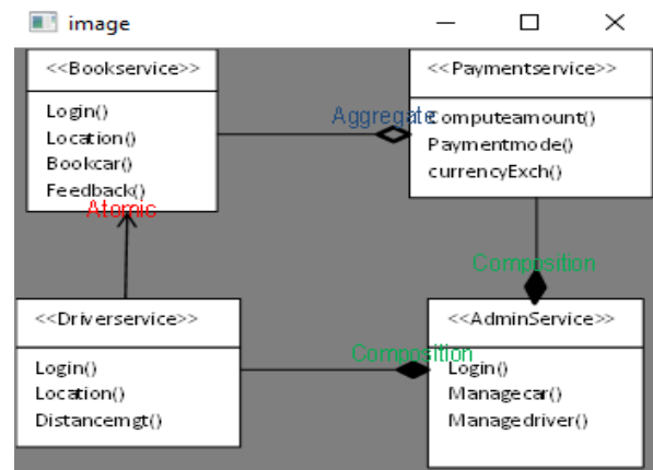
Figure 6: Arrow classification based on dependency
