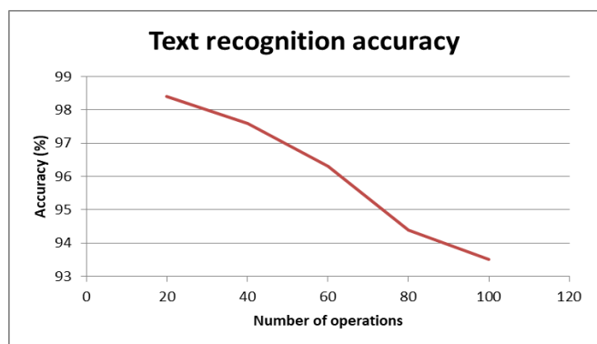
Figure 8: Text recognition accuracy
