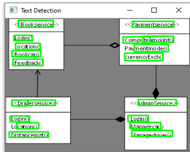
Figure 2: Detected text in UML interface
