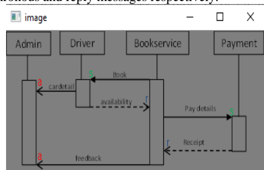
Figure 7: UML sequence diagram arrow classification
