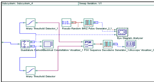
Figure -3 QPSK Demodulator
