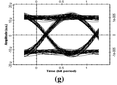
Figure -11: Eye Pattern with Dispersion compensation fiber, length 240 km, carrier at 400 MHz (a)-(c) ODSB (d)-(g) OSSB (a) & (d) Pre (b) & (e) Post (C) & (g) Symmetric
