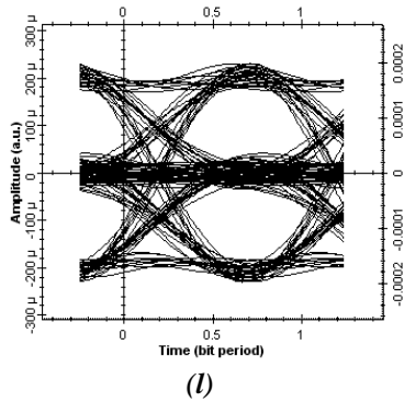
Figure -8: The Eye Patterns QPSK SCM Transmission Link (a)-(d) Back-to-Back (e)-(h) ODSB (i)-(l) OSSB
