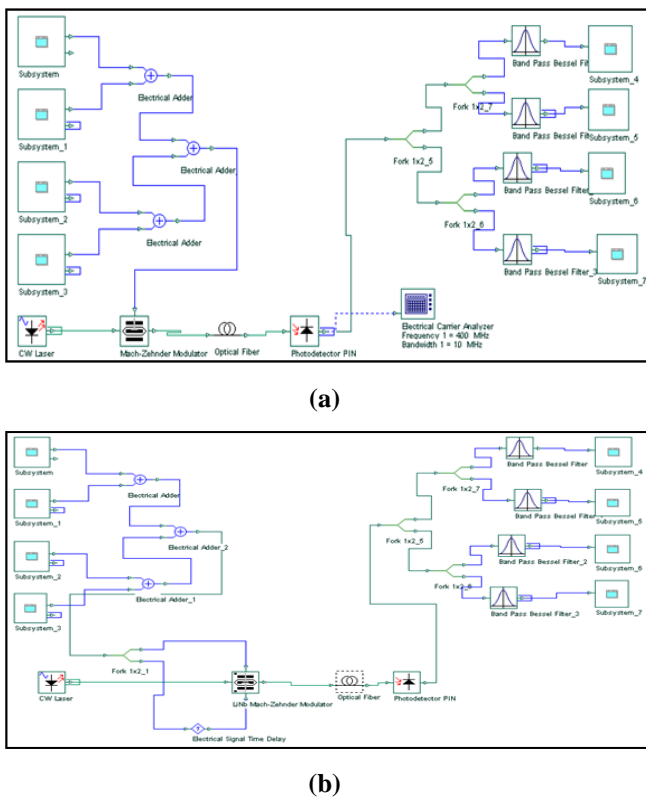
Figure -1: QPSK SCM Transmission Link (a) ODSB (b) OSSB
