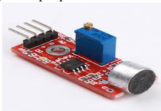
Fig. 2. LM-393 Sound Sensor.
