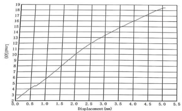
Fig. 4 Load vs Displacement curve of second sample
