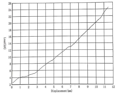
Fig. 7 Load vs Displacement curve for confined bamboo sample
