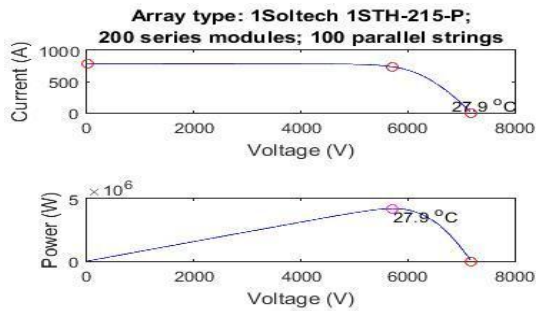
Fig. 2.Characteristics of Photovoltaic Array
