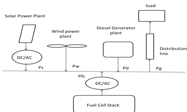
Fig. 1.schematic diagram of the hybrid system.
