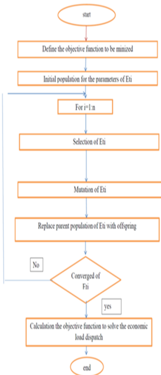
Fig. 6. flow chart of Economic load Dispatch (ELD)
