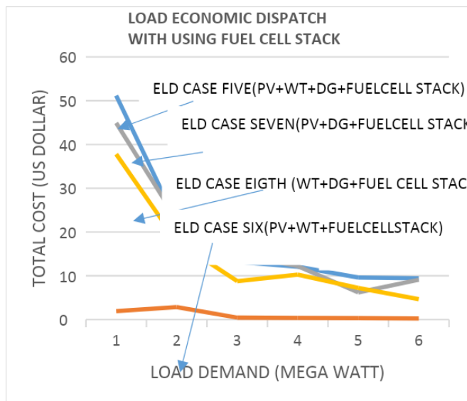
Fig. 9.load economic dispatch with using a fuel cell stack
