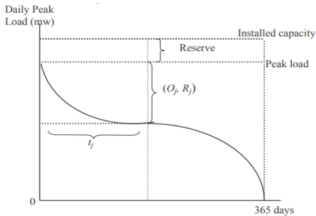
Fig. 7. Estimation of (LOLP) by load duration curve
