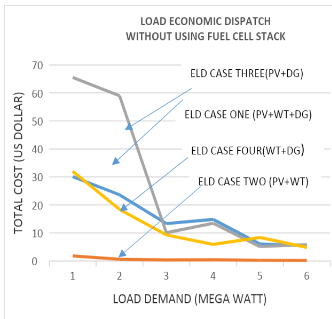
Fig. 8.load economic dispatch without using a fuel cell stack
