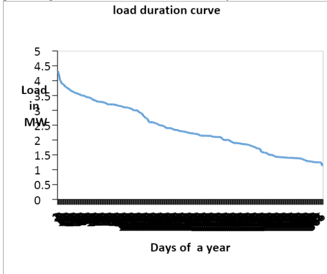
Fig. 10. Load duration curve of study area
