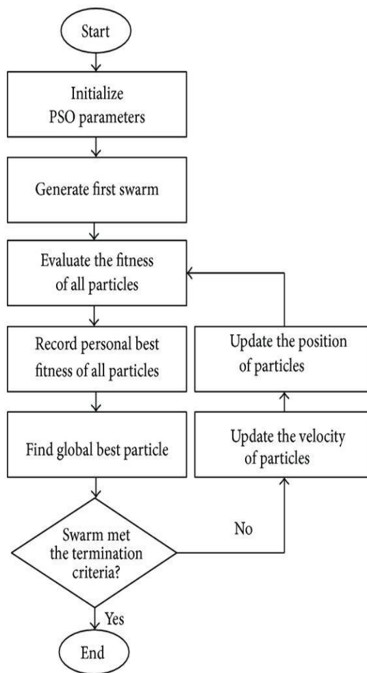
Fig. 5. The flow chart of partial swarm optimization
