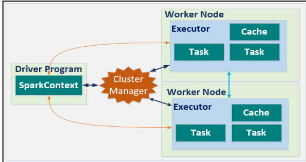
Fig. 5 (a): Apache Spark cluster architecture
