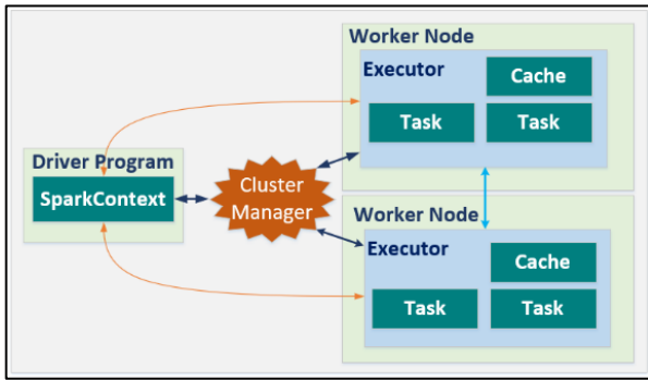
Fig. 5 (a): Apache Spark cluster architecture
