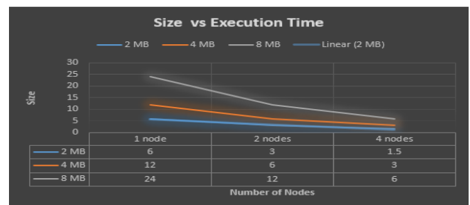
Fig. 6: Execution time on Apache Spark based system(s)
