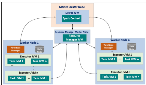
Fig. 5 (b): Apache Spark cluster architecture
