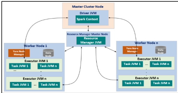
Fig. 5 (b): Apache Spark cluster architecture
