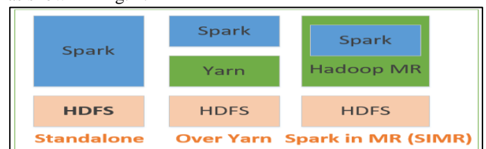
Fig. 4: Different methods of using Spark
