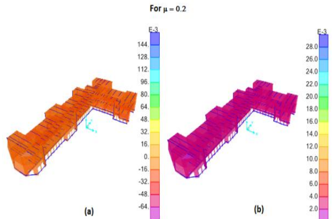
Fig. 7. (a) Direct Principal Stresses (MPa) due to seismic load in X and Y directions (b) Shear Stress (MPa) due to seismic load in X and Y directions.
