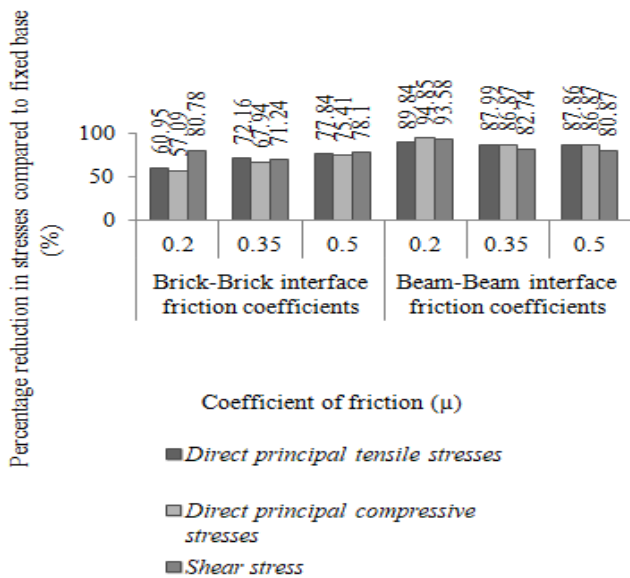
Fig. 8. Percentage reduction in stresses in X direction compared to fixed base.
