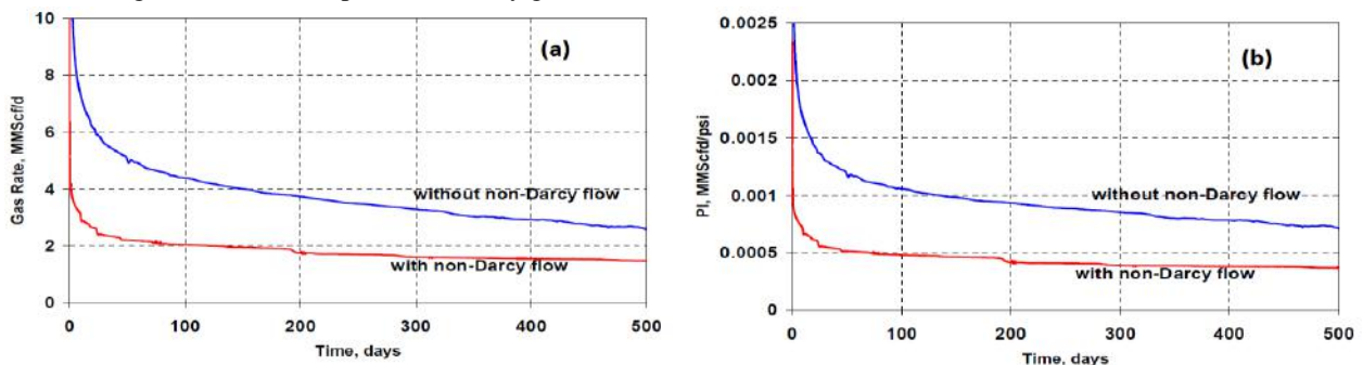
Fig. 5. Non-Darcy flow impact on a) Gas rate & b) Productivity index
