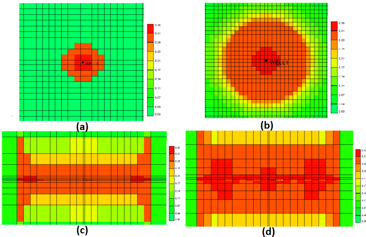
Fig. 3. Plan view of condensate saturation for a) “without fracture” after 800 days, b) “without fracture” after 3500 days, c) “with fracture” after 500 days & d) “with fracture” after 800 days
