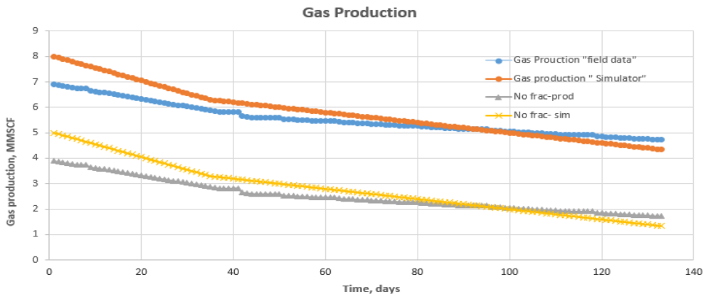
Fig. 4. Gas production log during 135 days for a) field data “with fracture”, b) simulator data “with fracture”, c) field data “without fracture” & d) simulator data “without fracture”
