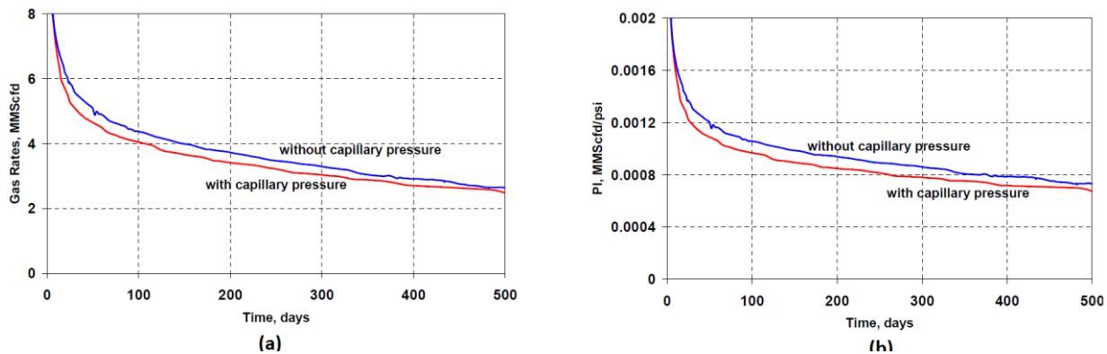
Fig. 7. Capillary pressure impact on a) Gas rate & b) Productivity index
