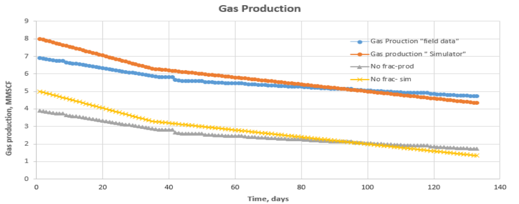
Fig. 4. Gas production log during 135 days for a) field data “with fracture”, b) simulator data “with fracture”, c) field data “without fracture” & d) simulator data “without fracture”
