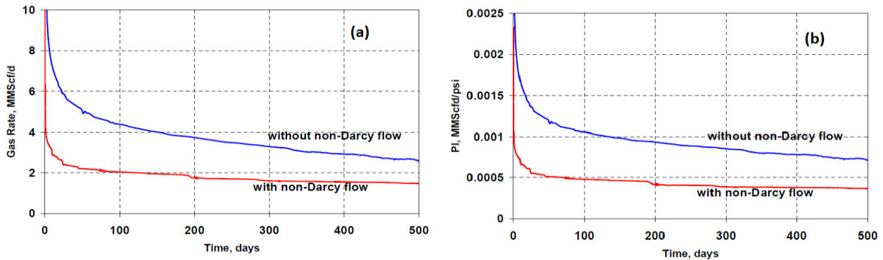
Fig. 5. Non-Darcy flow impact on a) Gas rate & b) Productivity index
