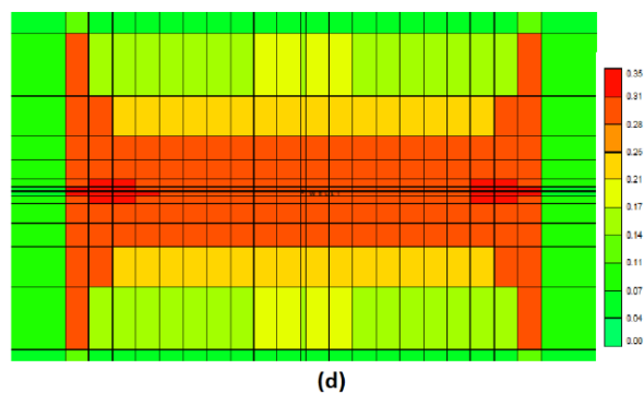
Fig. 6. Capillary number impact on a) Gas rate, b) Condensate rate. Plan view of condensate saturation around the fracture after 500 days c) without including capillary number & d) with including capillary number
