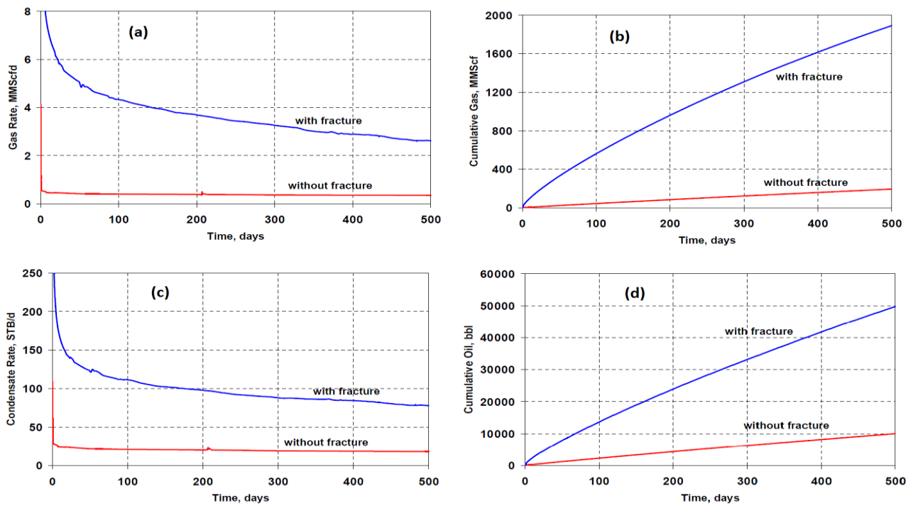
Fig. 2. Hydraulic fracture impact on a) Gas rate, b) Cumulative gas production, c) Condensate rate & d) Cumulative condensate production
