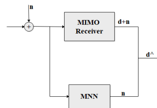
Fig.4. MNN Testing block diagram
