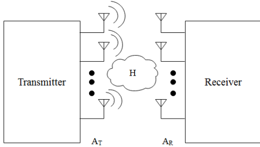
Fig. 1. Basic block diagram of MIMO
