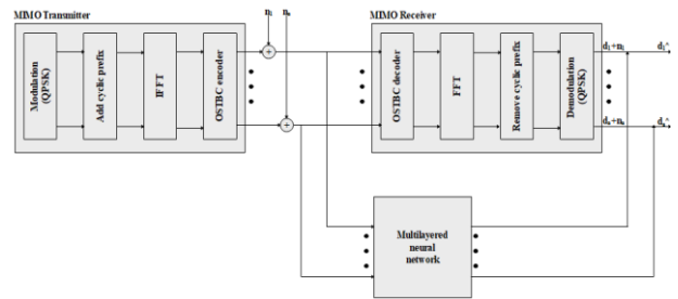
Fig.2. Block diagram of the ‘‘MNN-MIMO-CE’’ method
