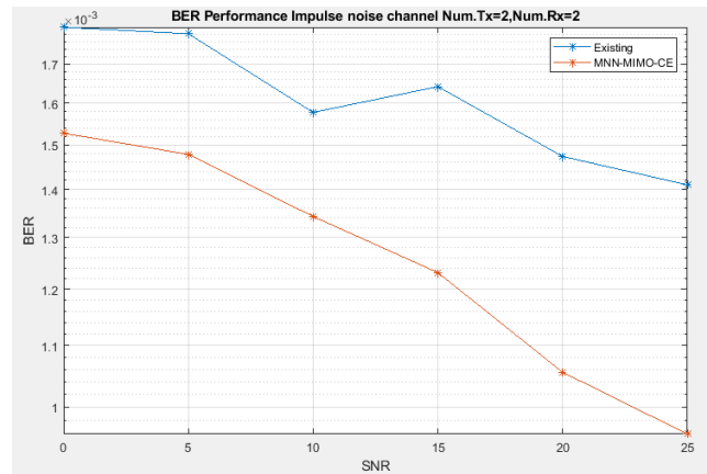
Fig.8.2x2MNN-MIMO-CE system comparison with the existing system [25] in impulse noise channel
