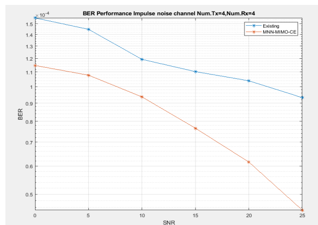
Fig 9.4x4 ANN-MIMO-DF system comparison with the existing system [25] in impulse noise channel.
