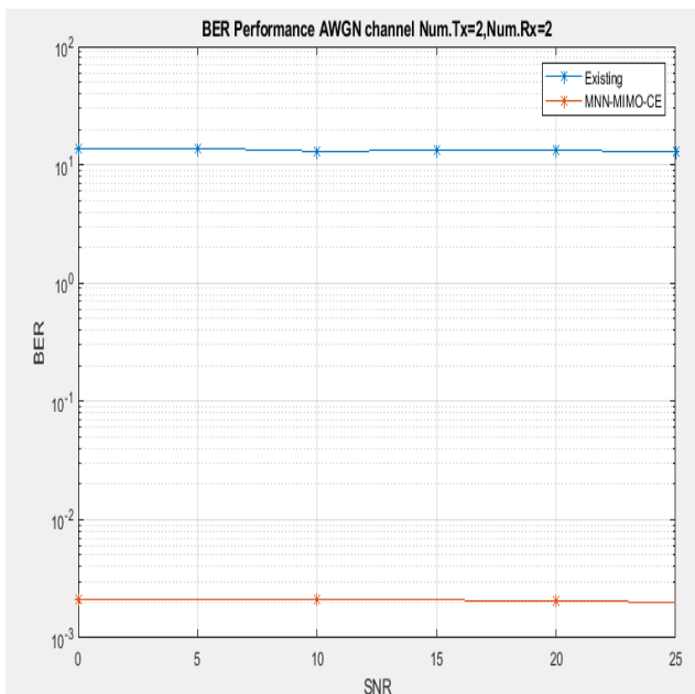
Fig.7.MNN-MIMO-CE system comparison with the existing system [25] in AWGN channel
