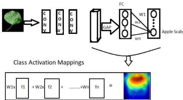
Fig.2 Architecture of CAM[7] B) Grad-Cam
