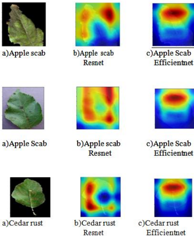
Fig.10 Shows the image of the leaf with plant and the othertwo images show how Grad-Cam was able to localize them after being attached to Resnet and Efficientnet
