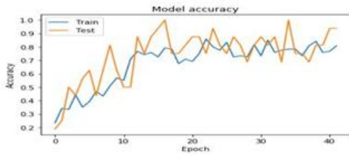
Fig.8 History of training Efficientnet with 60% training data and 40% testing data contains colored images accuracy
