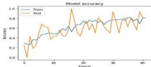
Fig.9 History of training Resnet with 60% training data and 40% testing data contains colored image Model accuracy
