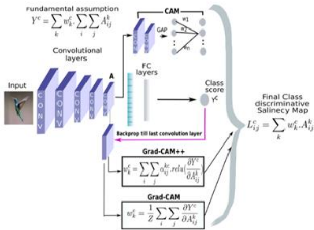
Fig.4 An overview of CAM, Grad-CAM and Grad-CAM++[9]
