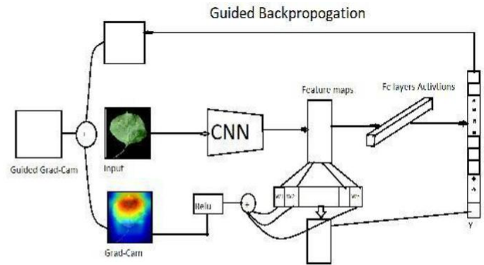
Fig .3 Architecture of Grad-Cam[8] C). Grad-Cam++
