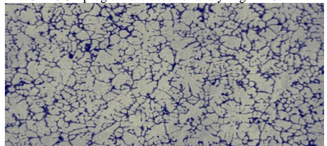
Fig.4.4.1 SPECIMEN A
