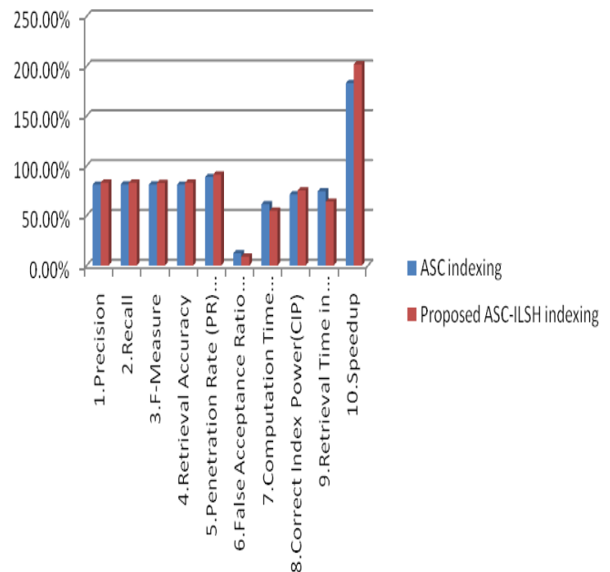
Fig. 4. Face Image Retrieval
