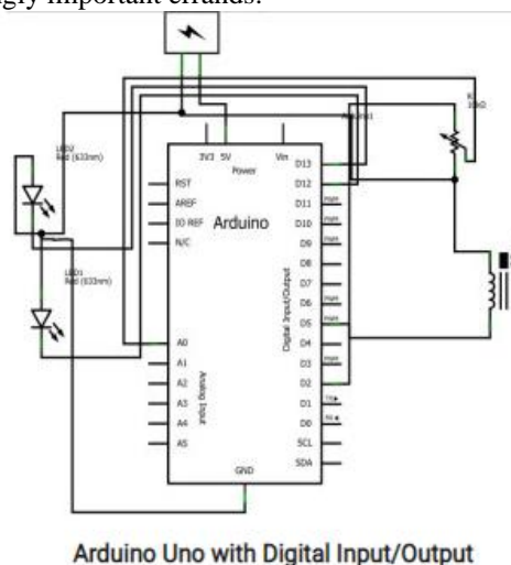
Fig 2: Arduino Board
