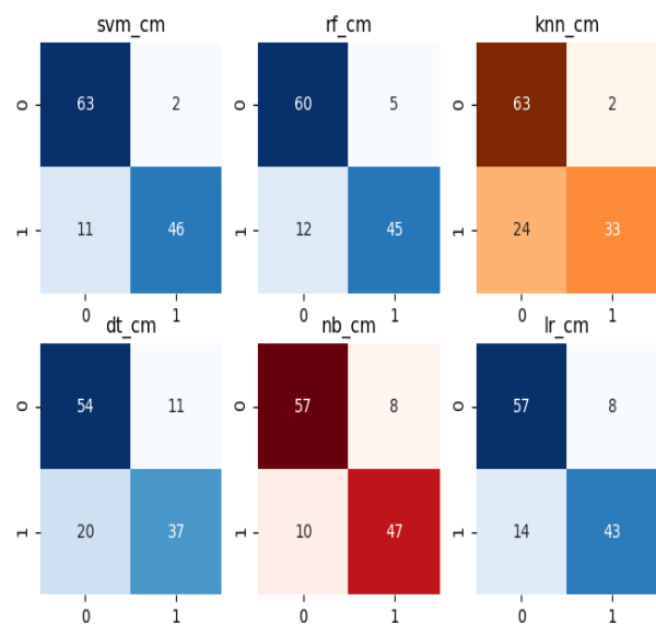
Figure 5: confusion matrix
