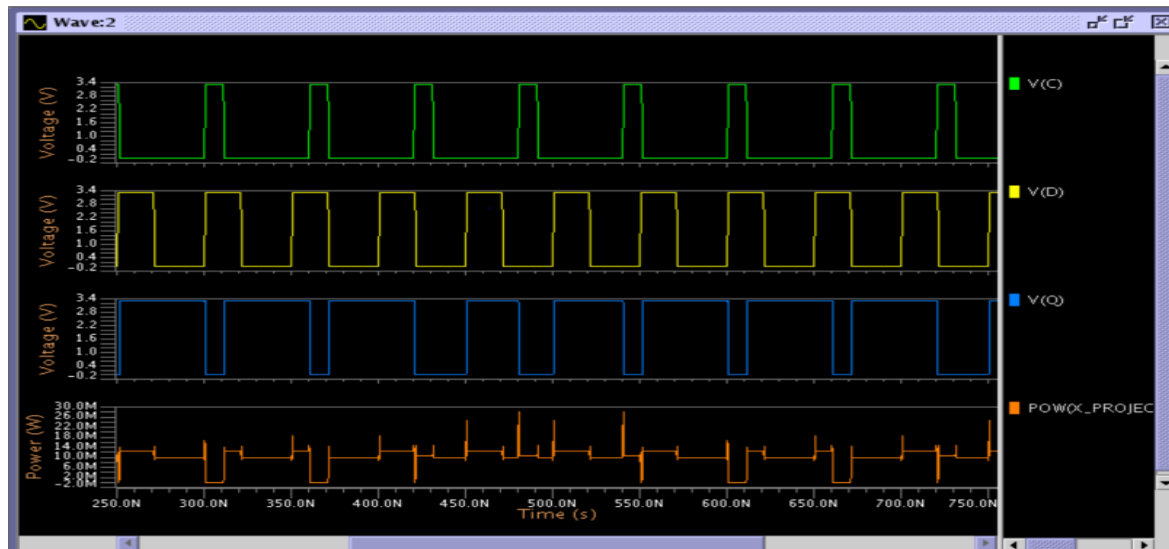
Fig: 4 Output Wave form of proposed technique showing glitch free output.
