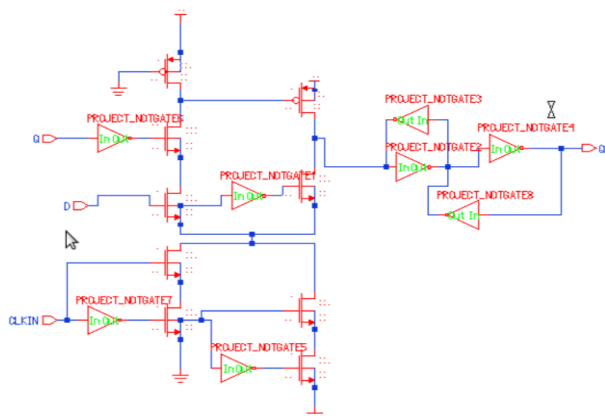
Fig.2 Latch Mux Flip flop using C-Element
