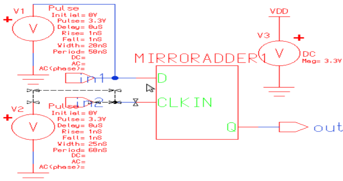
Fig: 6 Test Bench circuit of Latch Mux Flip flop considered for simulation
