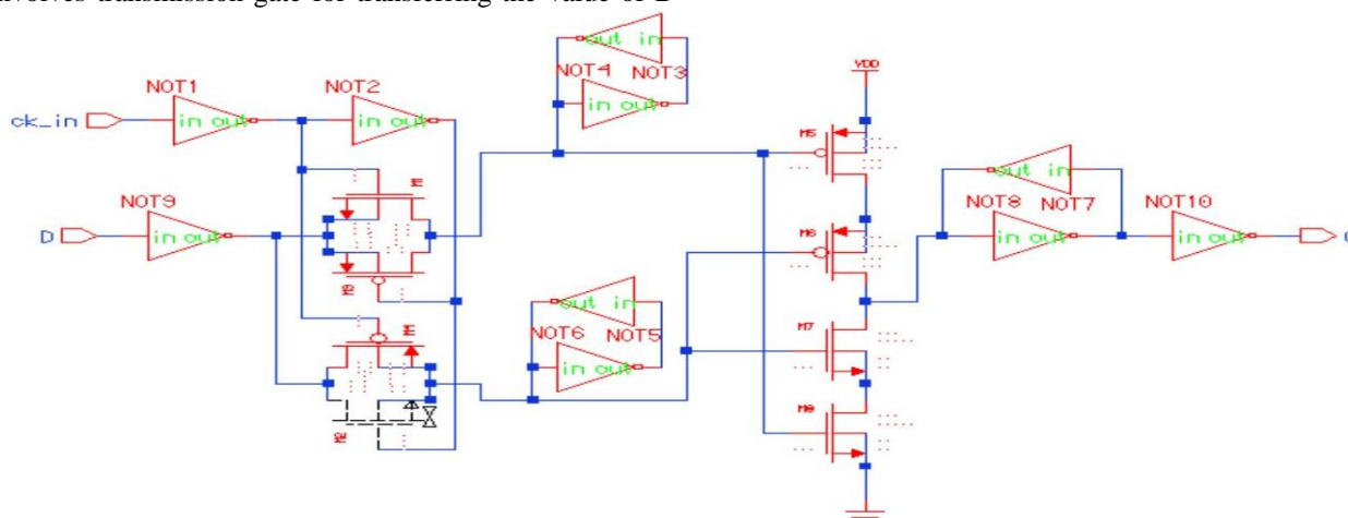
Fig.1 Latch Mux Flip flop
