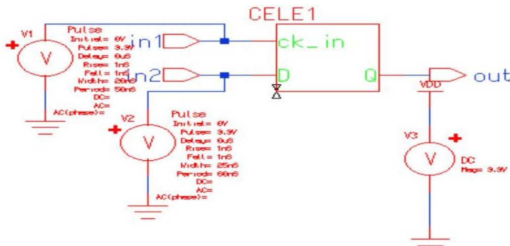
Fig: 5 Test Bench circuit of Latch Mux Flip flop using C-Element considered for simulation
