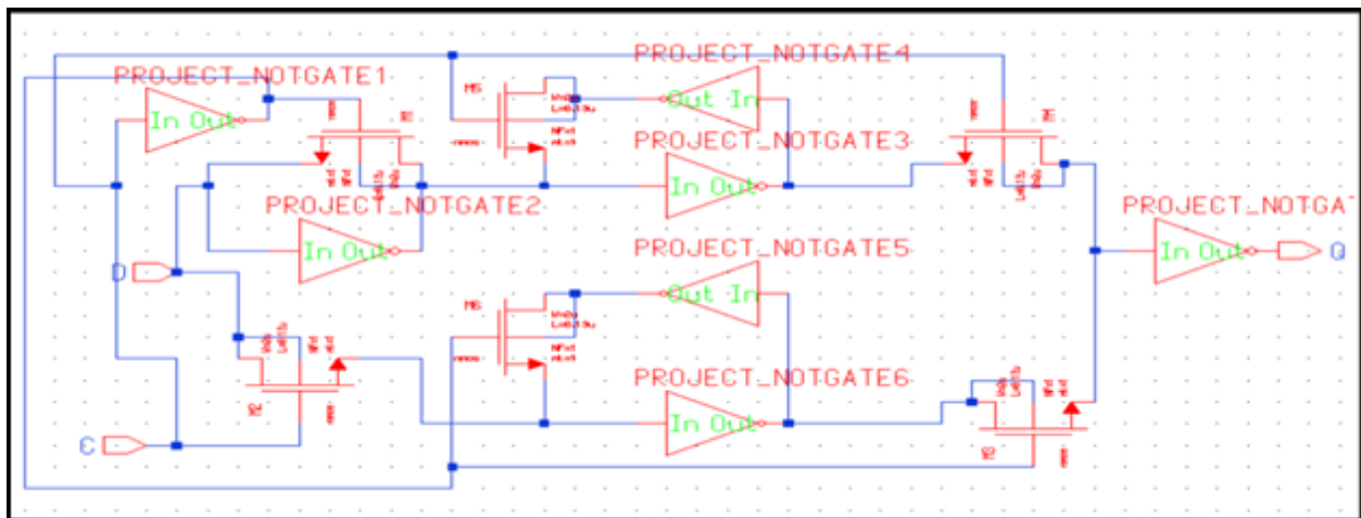
Fig.4 Proposed DET Flip Flop
