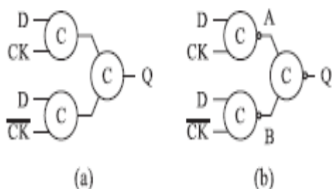
Fig: 2 Logic circuit of C-Element
