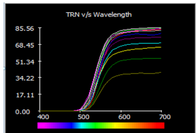
Fig 2: Transmission vs Wavelength curves of 5% Chitosan treated dye liquors
