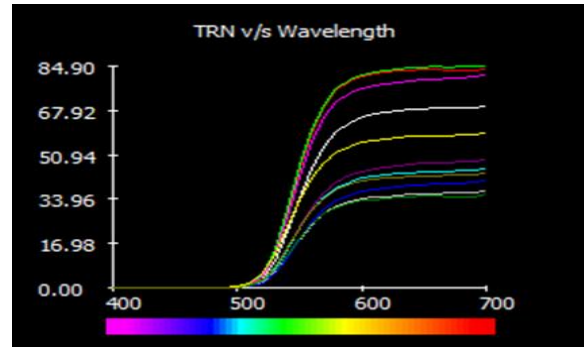
Fig 4: Transmission vs Wavelength curves of conventional dyed samples
