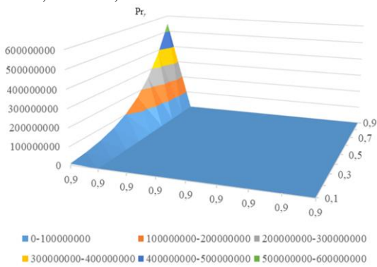
Fig. 2. The surface of the reseller's profit ( P_r ) provided that the equilibrium of the manufacturer by Stackelberg is formed at c_{am} = 0 , \beta = 0.9 , \alpha \in (0;1)
