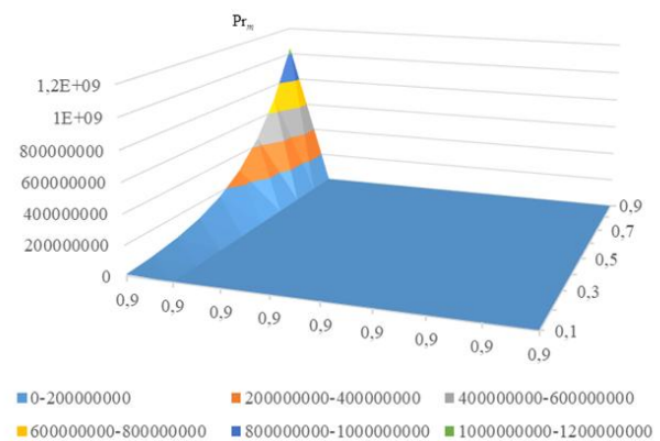
Fig. 1. Surface earnings manufacturer ( Pr_m ) provided by the manufacturer formation Stackelberg uilibrium, c_{am} = 0 , \alpha = 0,9 , \beta \in (0;1)
