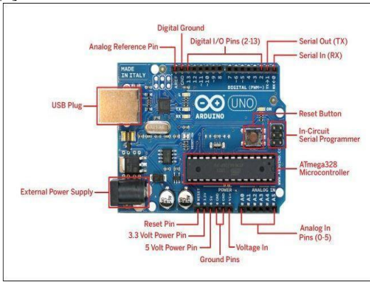
Fig. 4: Arduino Board
