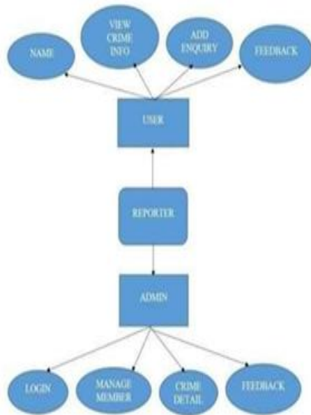
E-R Diagram
