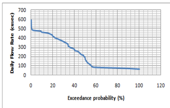
Fig. 7 Daily flow duration curve of Bukit Merah for Selinsing Canal in 2016
