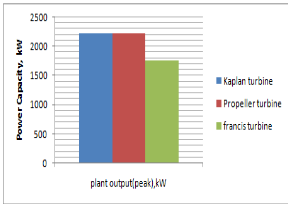
Fig. 9 Plant power capacities using different turbine types
