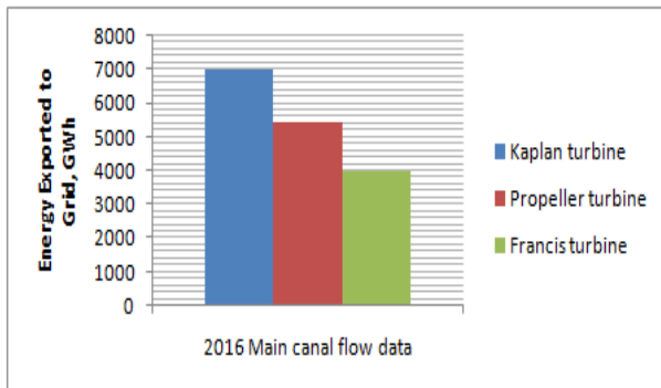
Fig. 10 Energy output using different turbine types
