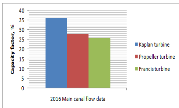
Fig. 11 Plant Capacity Factors using different turbine types
