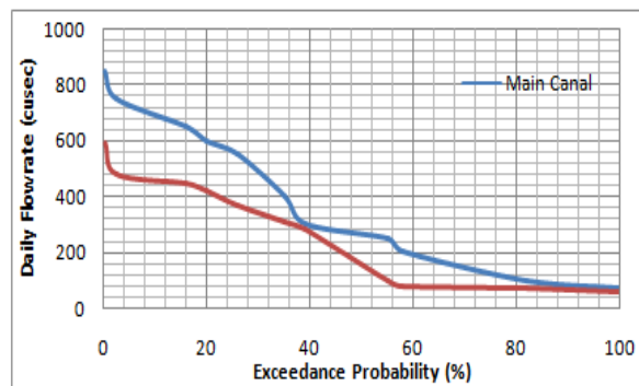
Fig. 8 Comparison of flow duration curve between the Main Canal and Selinsing Canal for 2016 daily flow rate data
