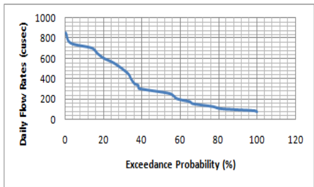
Fig. 6 Daily flow duration curve of Bukit Merah for Main Canal in 2016
