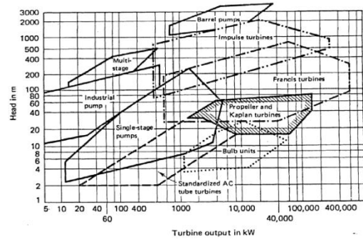
Fig. 4 Turbine Application Chart [8]
