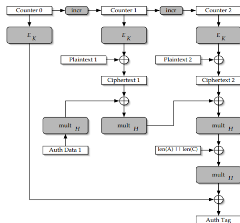
Figure 3: The authenticated encryption operation.
