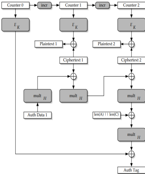
Figure 4: The authenticated decryption operation
