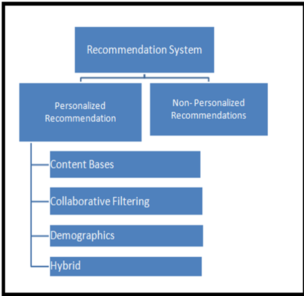
Fig. 3. Recommendation Techniques/Approaches
