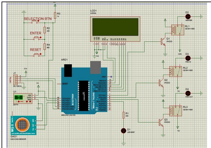
Fig. 5. Project simulation circuit
