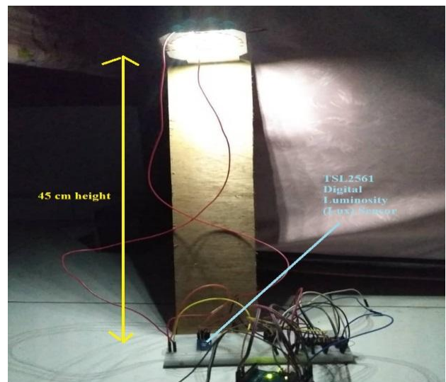
Fig. 7. PWM-LUX experiment setup
