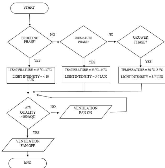
Fig. 2. Overall Project Operation Flowchart
