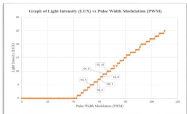
Fig. 8. Relationship between PWM and LUX
