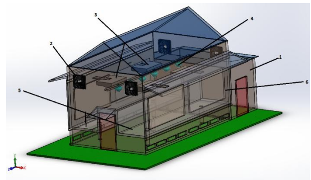
Fig. 4. Project prototype design.
