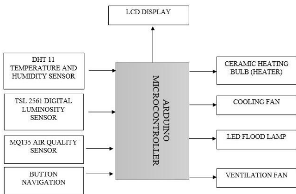
Fig. 1. Block diagram of Project IO declaration
