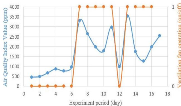
Fig. 10. Recorded AQI and Ventilation System Operation
