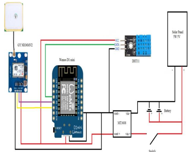
Figure 5. Hardware Connection for iBees's Device
