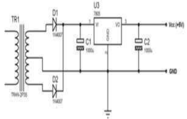
Fig 2: Power supply circuitry
