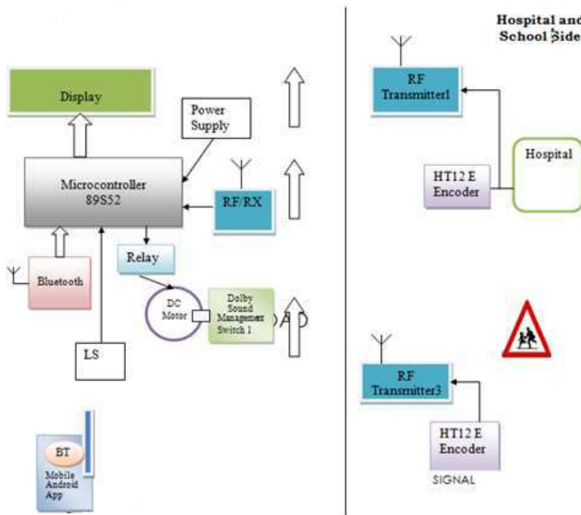
Fig 1: Block diagram
