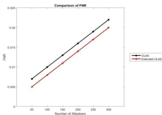
Fig.2: Comparison of FNR
