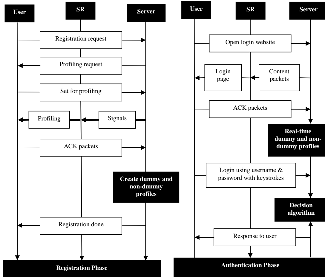
Fig.1: Extended CLAS Authentication Flowchart
