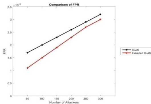
Fig.3: Comparison of FPR
