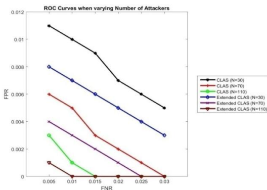
Fig.6: Comparison of ROC when varying Number of Attackers
