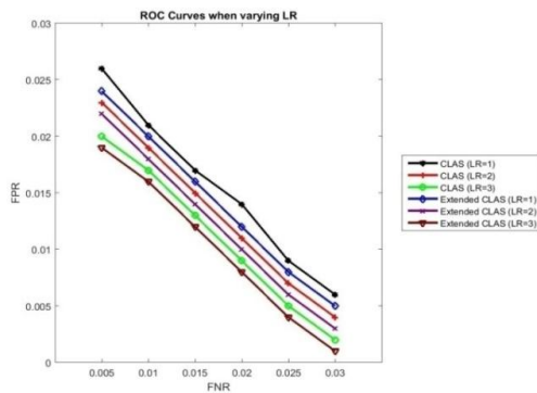
Fig.8: Comparison of ROC when varying LR
