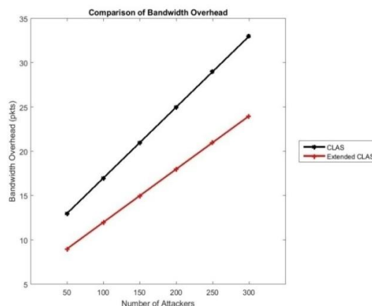
Fig.5: Comparison of Bandwidth Overhead
