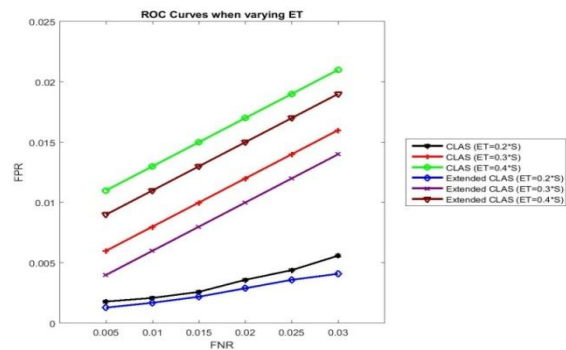
Fig.7: Comparison of ROC when varying ET
