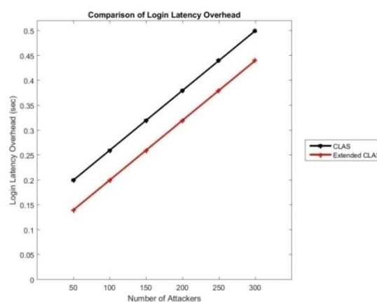
Fig.4: Comparison of Latency Overhead
