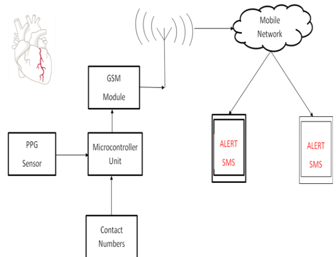
Fig 2. System Design
