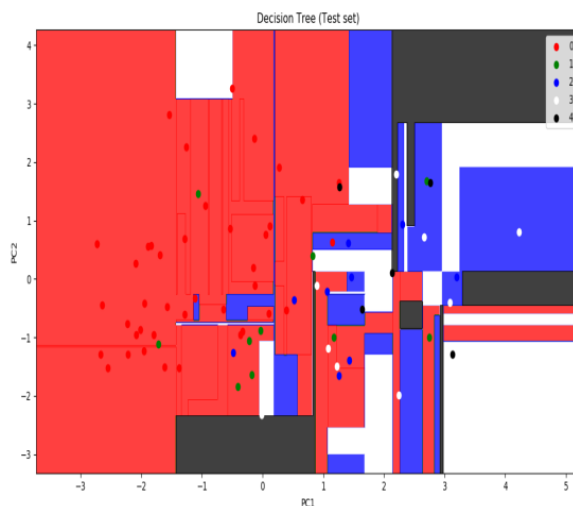
Fig-4.2 DecisionTree(Testset)
