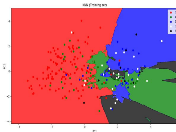
Fig-5.1 Nearestneighbour(Trainingset)
