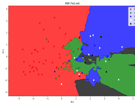
Fig-5.2 K-Nearestneighbour(Testset)
