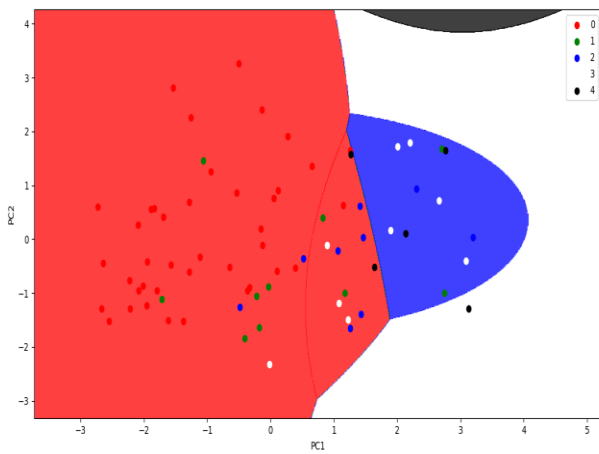
Fig-6.2 NaiveBayes(Testset)
