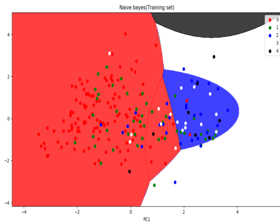
Fig-6.1 NaiveBayes(Trainingset)
