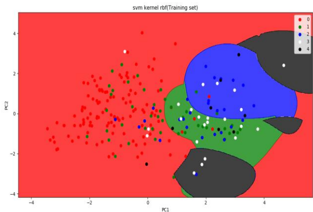
Fig-9.1 SVMRBF(Trainingset)
