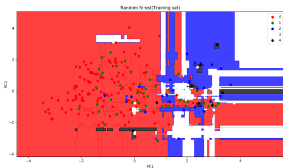
Fig-7.1 RandomForest(Trainingset)
