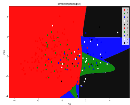
Fig-8.1 SVMPoly(Trainingset)
