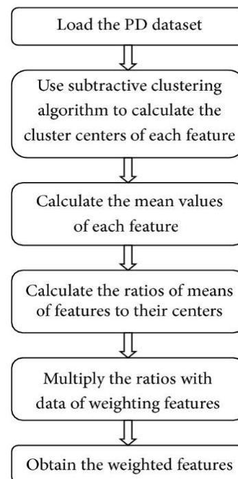
Figure 4.illustration of proposed overview with KMedoids algorithm.
