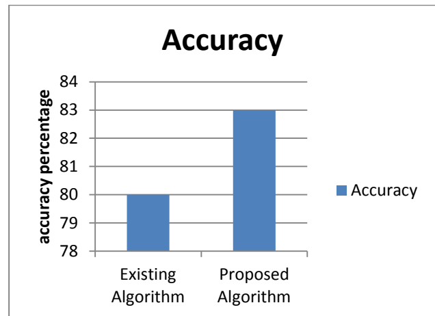
Fig 2: Accuracy Comparison
