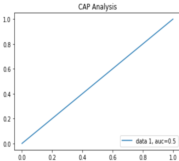
Fig 3: CAP Analysis
