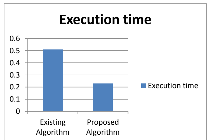
Fig 3: Execution time
