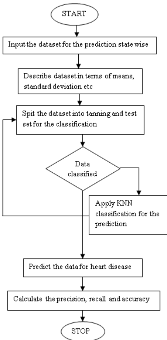
Fig 1: Proposed Methodology
