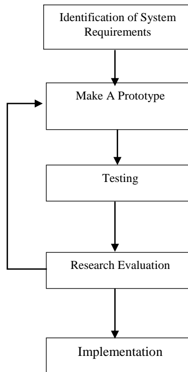
Fig. 2: Prototype Method
