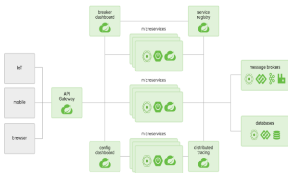
Fig. 1: Framework Architecture
