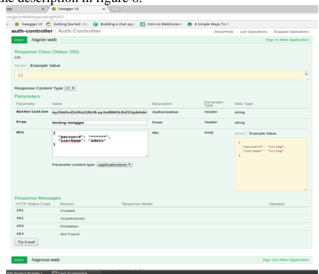
Fig. 8: Post Method.
