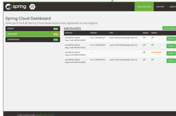
Fig. 3: Backend Analysis
