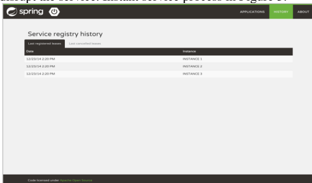
Fig. 5. Instant Service
