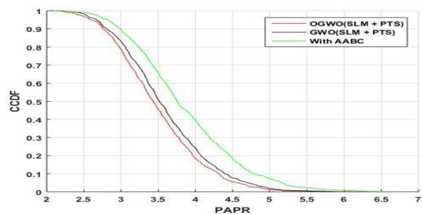
Figure 6. Comparison of PAPR vs. CCDF for proposed and existing methodologies
