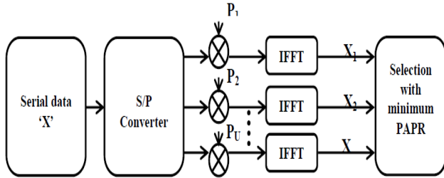
Figure 2: Block diagram of SLM
