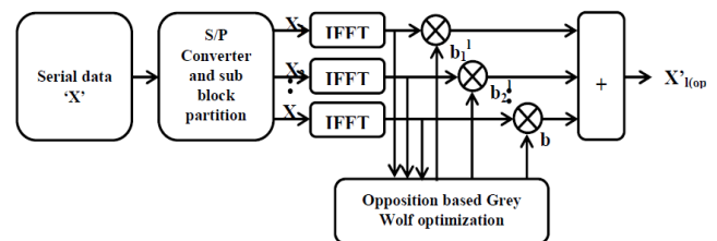
Figure 1. Block diagram of PTS
