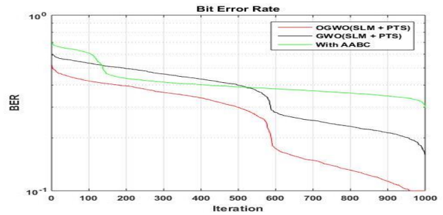
Figure 4. BER for proposed and existing methodologies
