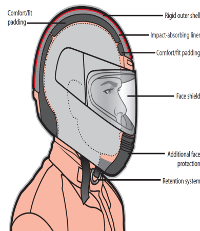
Fig 1: The basic constructions of helmet
