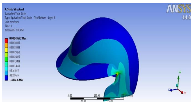
Fig 25: Shows the strain on Kevlar composite helmet for the load of 2000N
