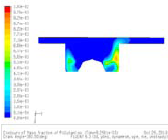
Fig 4 NOx formation
