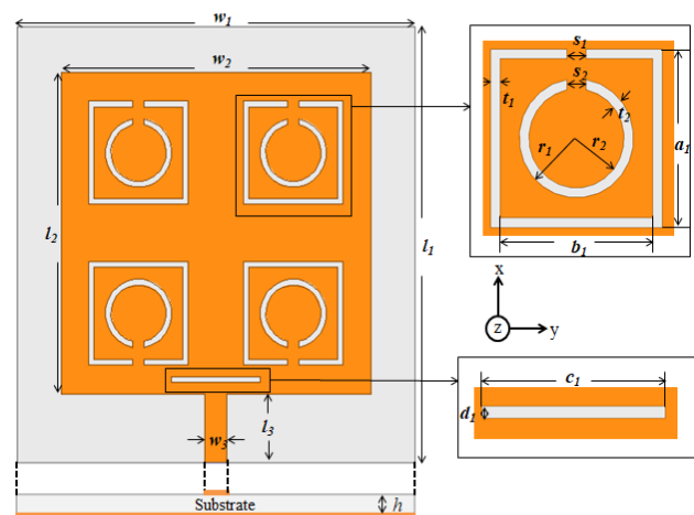
Figure 1. The proposed patch antenna geometry
