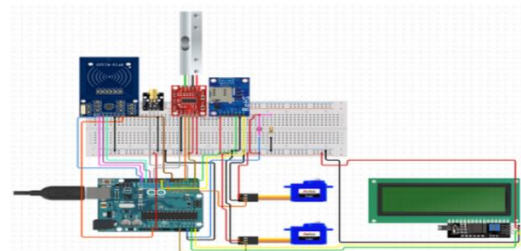
Figure 2. Simulation Diagram in Circuit.IO Software
