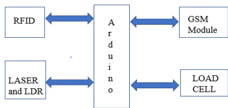
Figure 1. Block Diagram of the Proposed System
