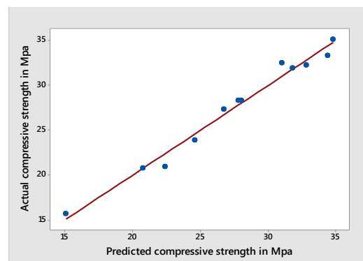
Figure 4 Actual values of CS Vs Predicted values of CS.
