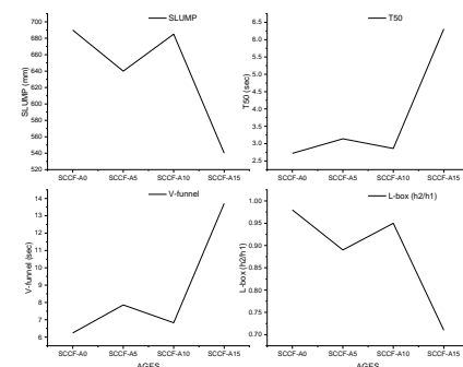
Figure 1 Fresh properties of SCC
