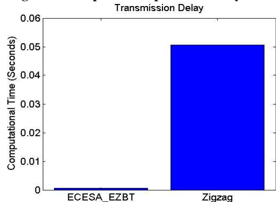
Figure 7: comparison of transmission delay
