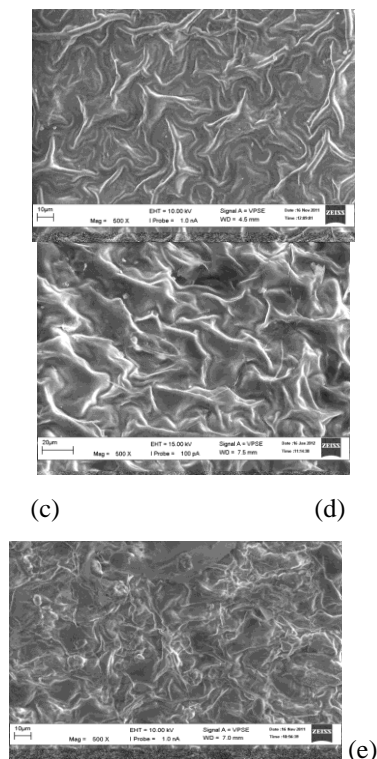
Fig 2. The surface of plant matrix at various solvent a) before extraction b) water, c) acetone, d) acetonitrile, e) ethanol. Magnification 500x.
