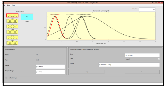
Fig.11. Fuzzification of selected input features using MF obtained using SCG training algorithm.
