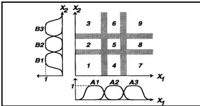
Fig.3. Example of K-means clustering used to form fuzzy sets for two features and three classes
