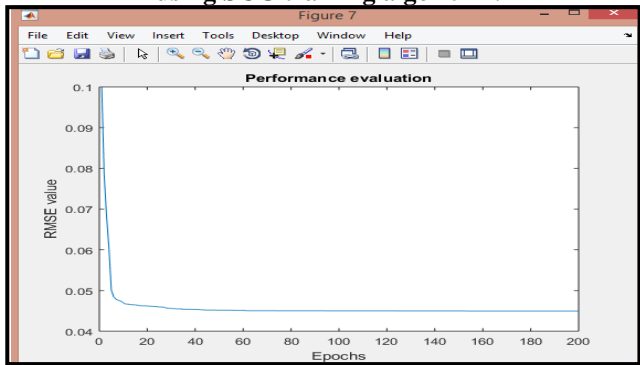
Fig.8. Graph of RMSE verses number of epoch while obtaining MF using SCG training algorithm.
