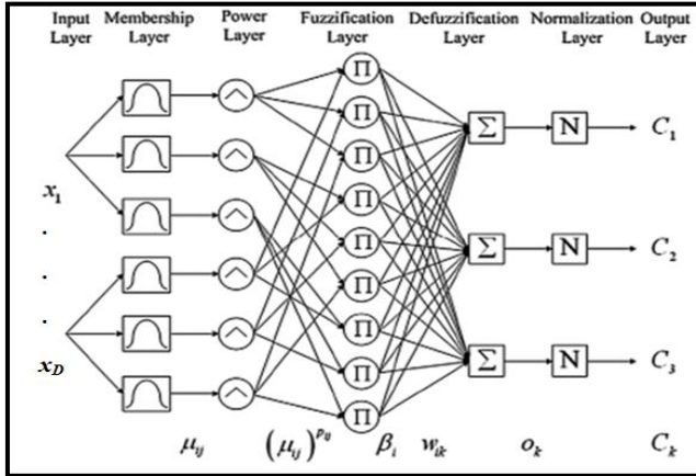
Fig.4. Architecture of Neuro-Fuzzy Classifier
