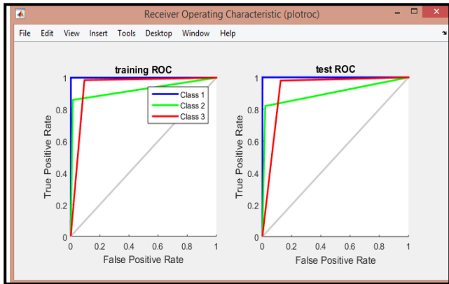
Fig.15. ROI plots obtained for training and test sets applied to Neuro-fuzzy Classifier.
