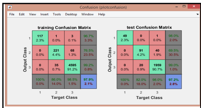
Fig.14. Confusion Matrices obtained for training and test sets applied to Neuro-fuzzy Classifier.
