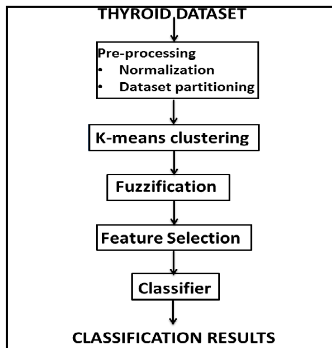
Fig.1. Flowchart of Proposed Neuro-Fuzzy Approach.
