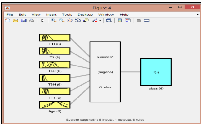
Fig.10. Model representation of Neuro-fuzzy system with selected features.
