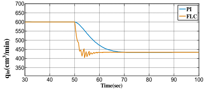
Fig.20. Response of PI and FLC output ( q_{in} ) for load variation in +6% from q_{L1} .
