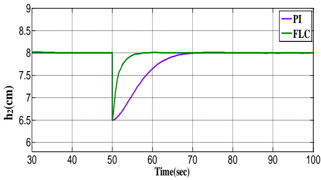
Fig.15. Regulatory response of h_2 with PI and FLC due to load variation in -6% from q_{L2} .
