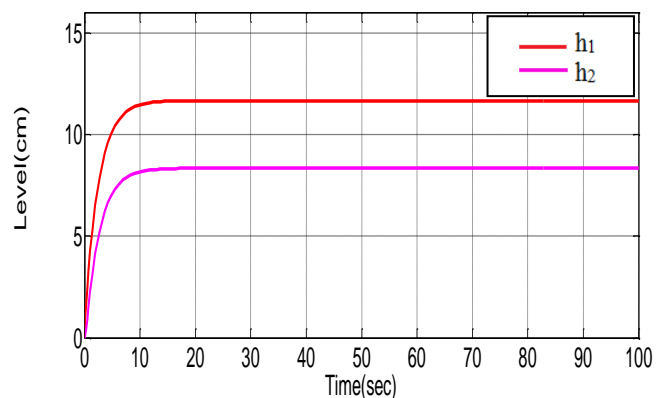
Fig.5. Simulated open loop response of h_1 and h_2 of interacting Process.
