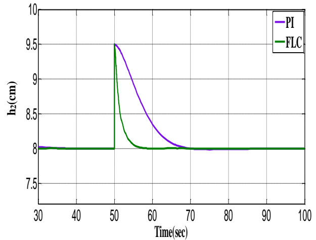
Fig.12. Regulatory response of h_2 with PI and FLC due to load variation in +6% from q_{L2} .
