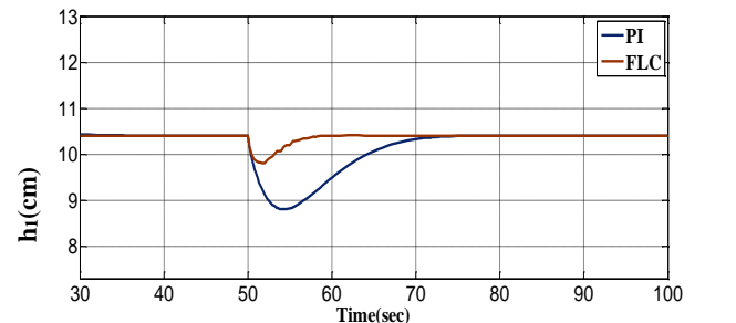
Fig.22. Regulatory response of h_1 with PI and FLC due to load variation in -6% from q_{L1} .
