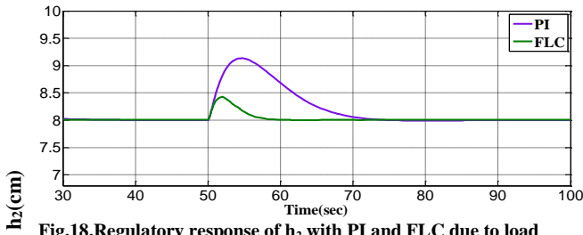
Fig.18. Regulatory response of h_2 with PI and FLC due to load variation in +6% from q_{L1} .
