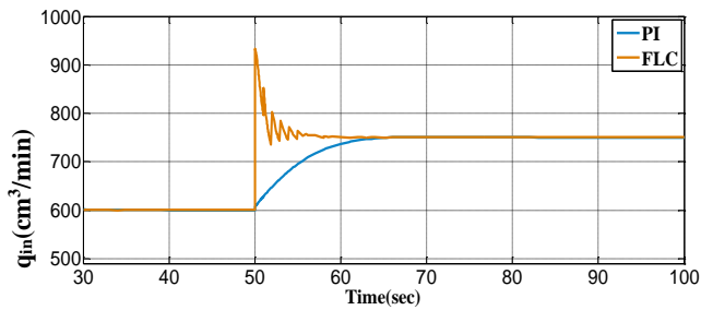
Fig.17. Response of PI and FLC output ( q_{in} ) for load variation in -6% from q_{L2} .
