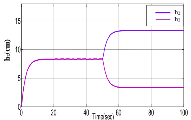
Fig.6.Simulated PRC of h_2 for step change in q_{in} for \pm 499.8 cm 3 /min.
