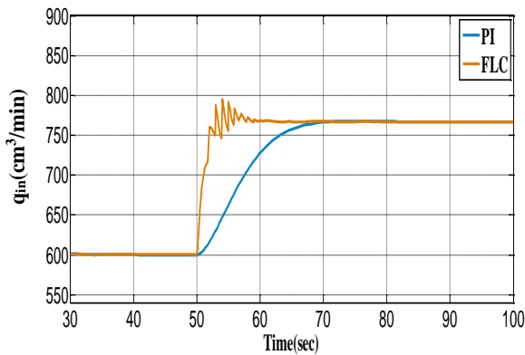
Fig.23. Response of PI and FLC output( q_{in} ) for load variation in -6% from q_{L1} .
