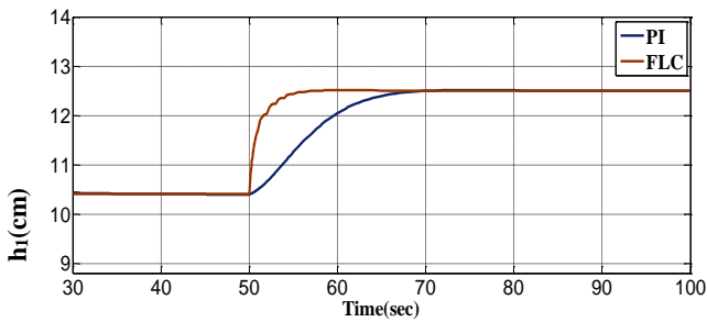
Fig.16. Regulatory response of h_1 with PI and FLC due to load variation in -6% from q_{L2} .
