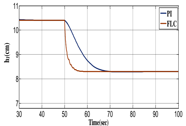
Fig.13. Regulatory response of h_1 with PI and FLC due to load variation in +6% from q_{L2} .
