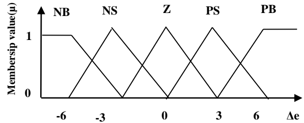
Fig.8(b). Membership diagram for change in error.
