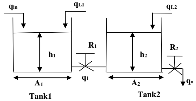
Fig.2.Two-tank interacting process.
