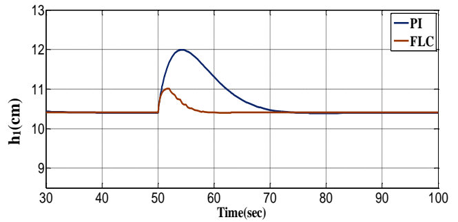
Fig.19. Regulatory response of h_1 with PI and FLC due to load variation in +6% from q_{L1} .
