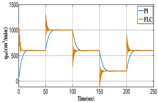
Fig.11. Response of PI and Fuzzy Logic Controller output ( q_{in} ) for servo response.
