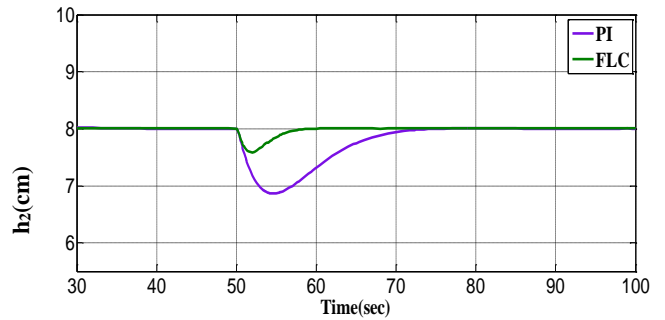
Fig.21. Regulatory response of h_2 with PI and FLC due to load variation in -6% from q_{L1} .
