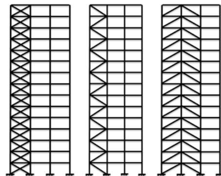
Fig. 3 Section of Brace Frame
