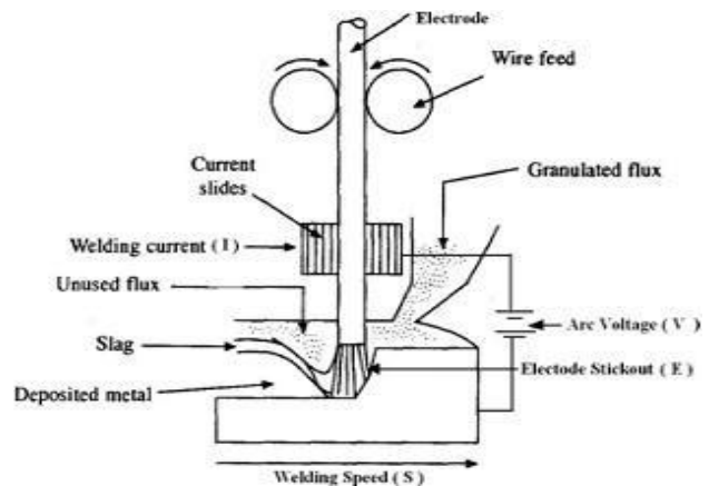
Figure 1: Submerged Arc Welding Process (Figure adopted from reference [1])
